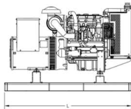
Open: (inches) 62L x32W x48H
